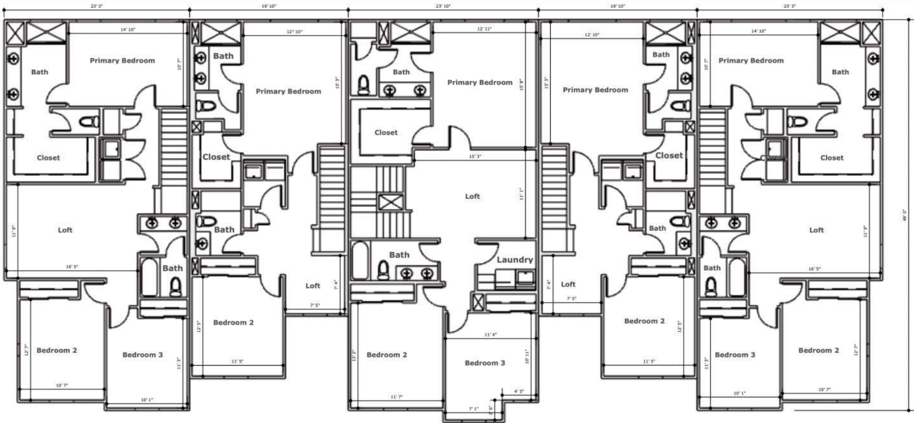
SECOND LEVEL
