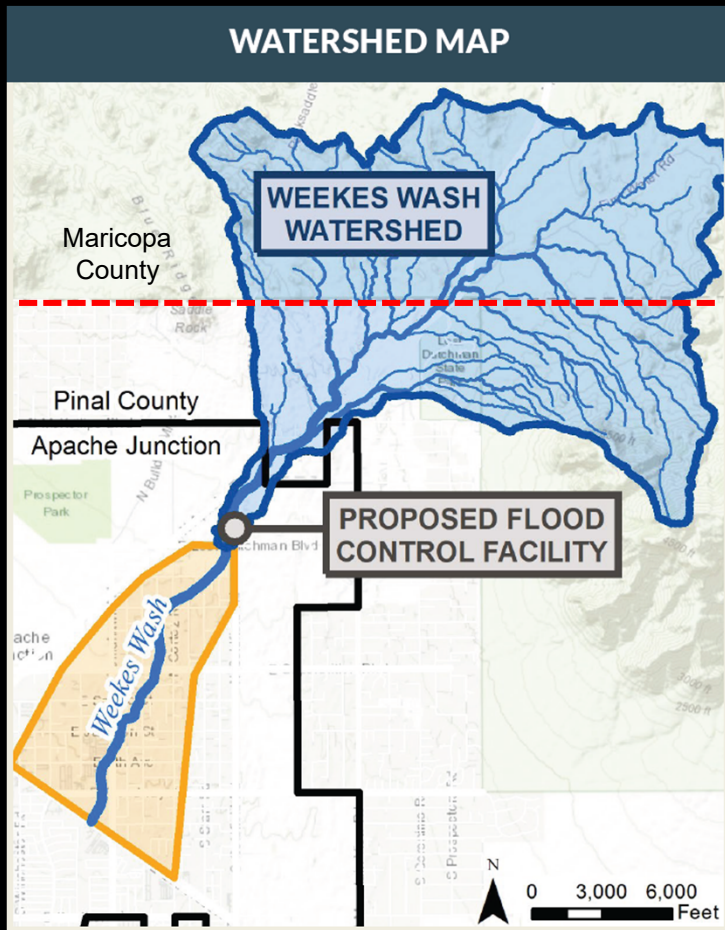
Weekes Wash Regional Flood Control Facility
