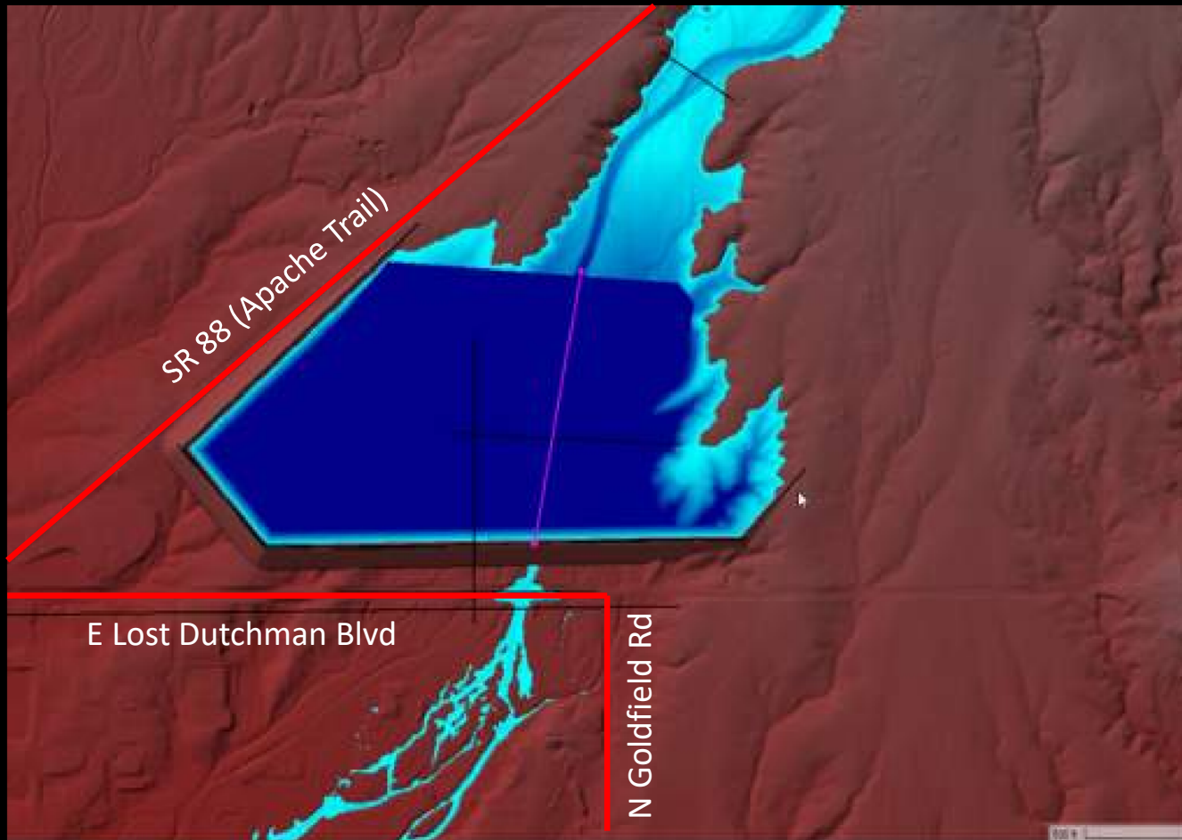
Weekes Wash Regional Flood Control Facility
