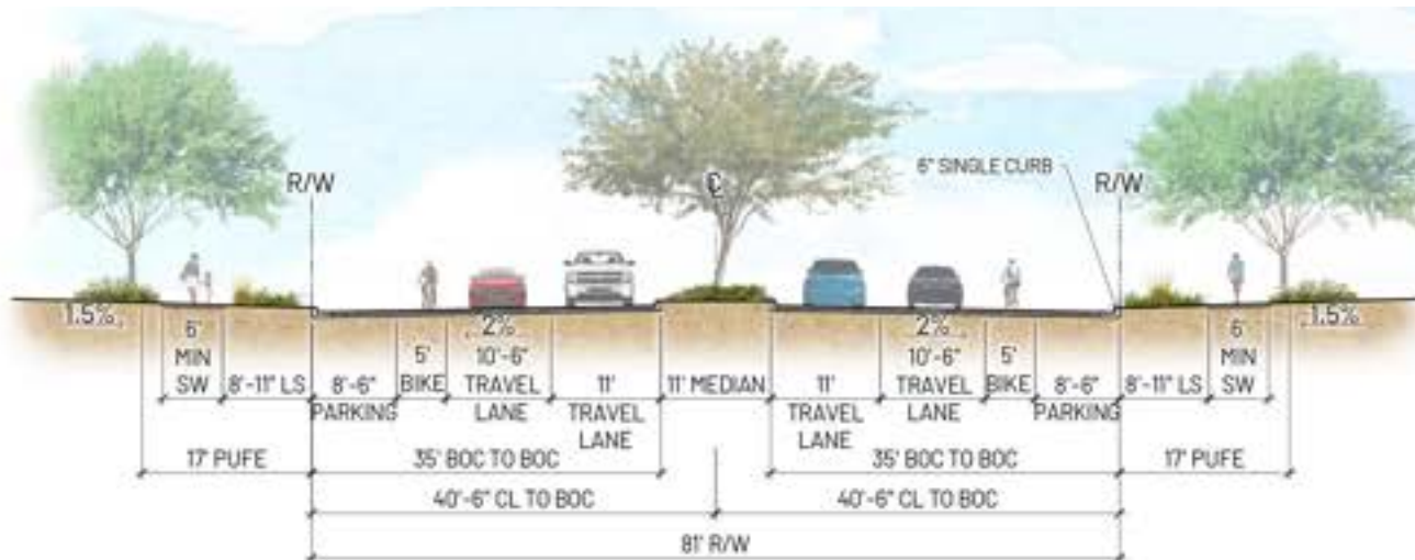
G 81' MAJOR COLLECTOR STREET (RAISED MEDIAN WITH ON STREET PARKING) SCALE: 1"=10'-0" PARKING ON BOTH SIDES DETACHED SIDEWALK *STRIPED MEDIAN FOR TURN LANES
