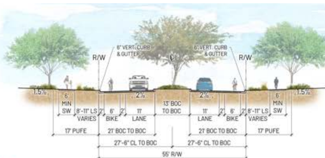
H 55' MINOR COLLECTOR STREET (RAISED MEDIAN) SCALE: 1"=10'-0" NO PARKING DETACHED SIDEWALK
